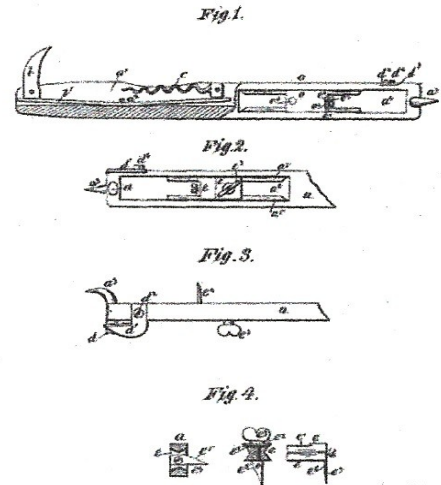
(Model.) I. N. ARMENT. CAN OPENER. No. 327,923. Patented Oct. 13, 1885.
