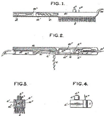
(Model.) I. N. ARMENT. Opener for Cans and Bottles. No. 234,646. Patented Nov. 23, 1880.
