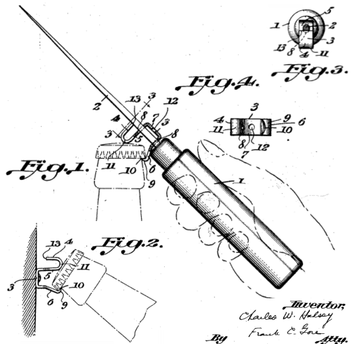
Dec 31, 1929. C. W. HALSEY 1,741,294 Bottle Cap Lifter Filed Oct. 15, 1928
